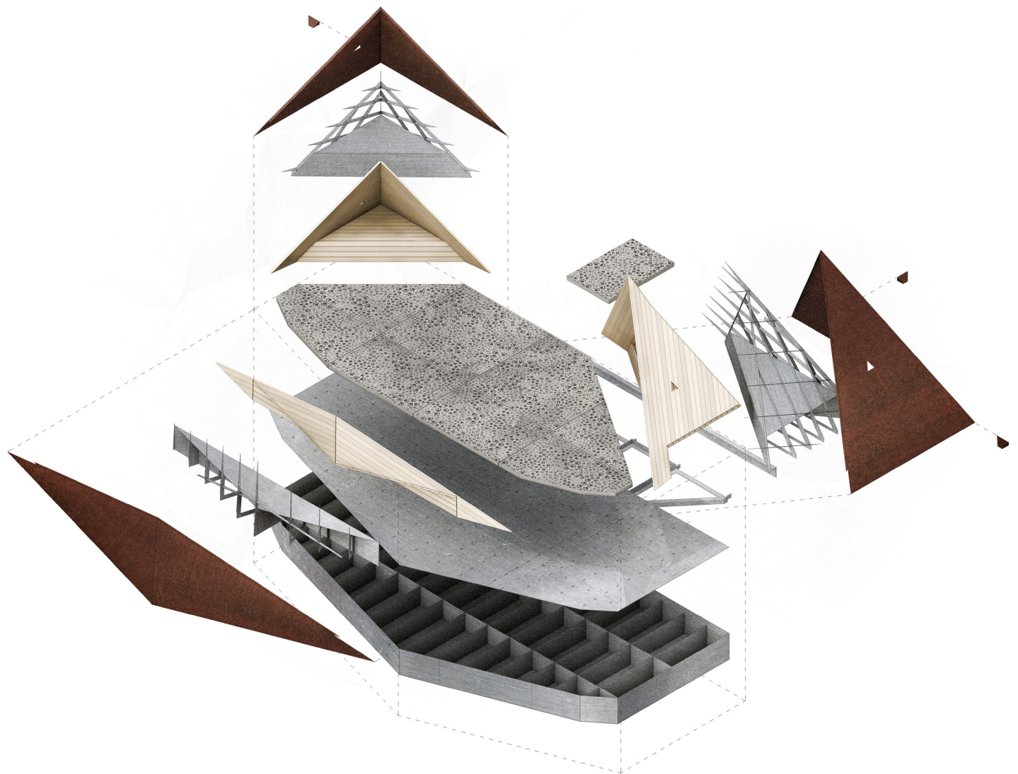
Axometric drawing of the structure
