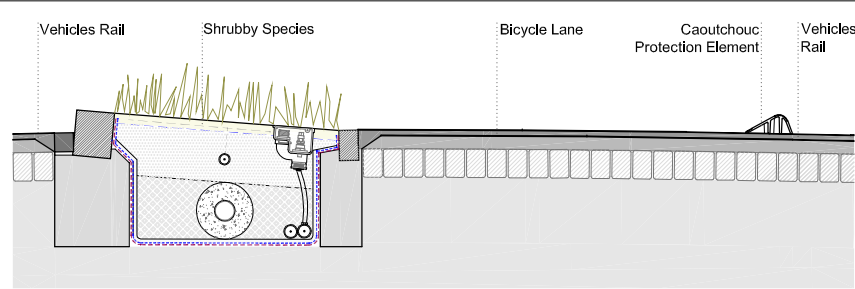
BICYCLE LANE-PLANTS PARTERRE CROSS SECTION
