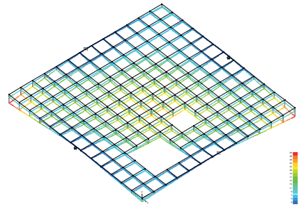
Structural schemes
