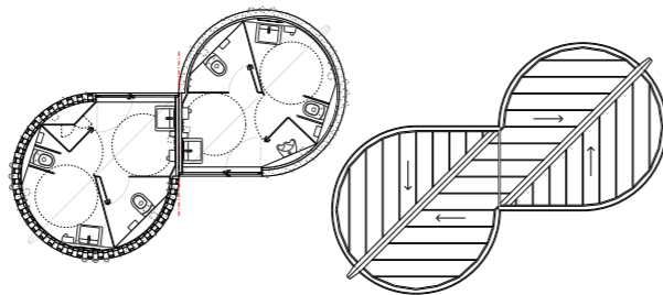
Plans of the kiosks for toilets
