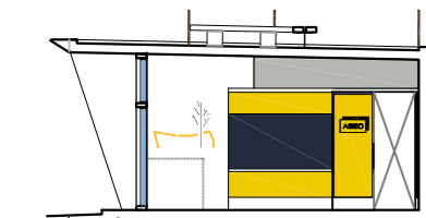
section b
